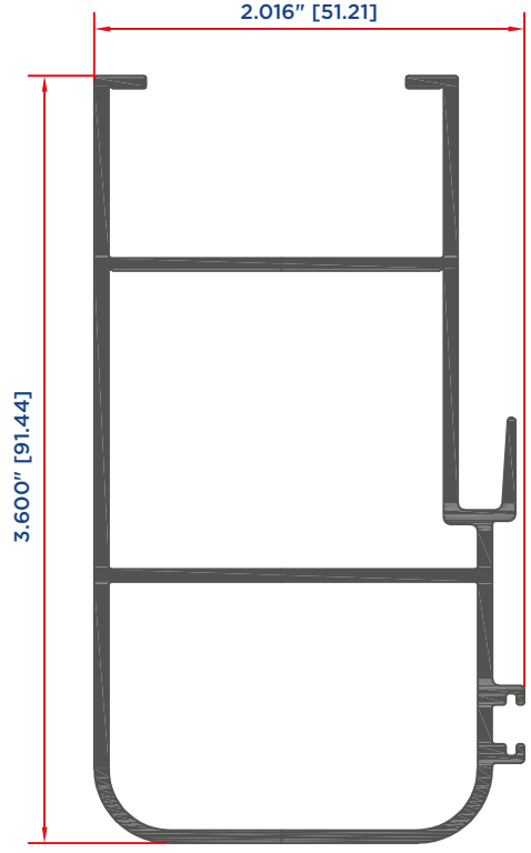
TRASLAPE DUO 12312
