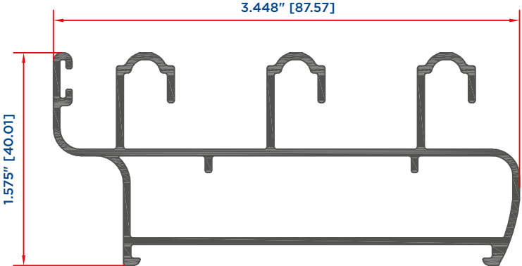
RIEL TRIPLE 1694
